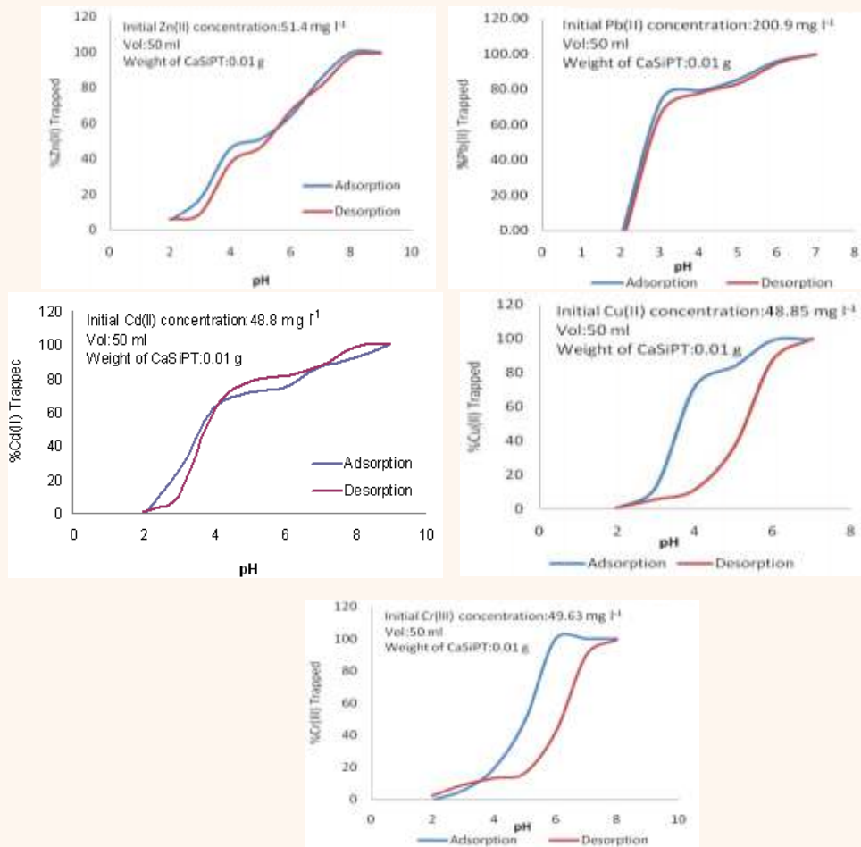
Fig.5. Adsorption–desorption hysteresis of Zn(II), Pb(II), Cd(II) Cu(II) and Cr(III)
