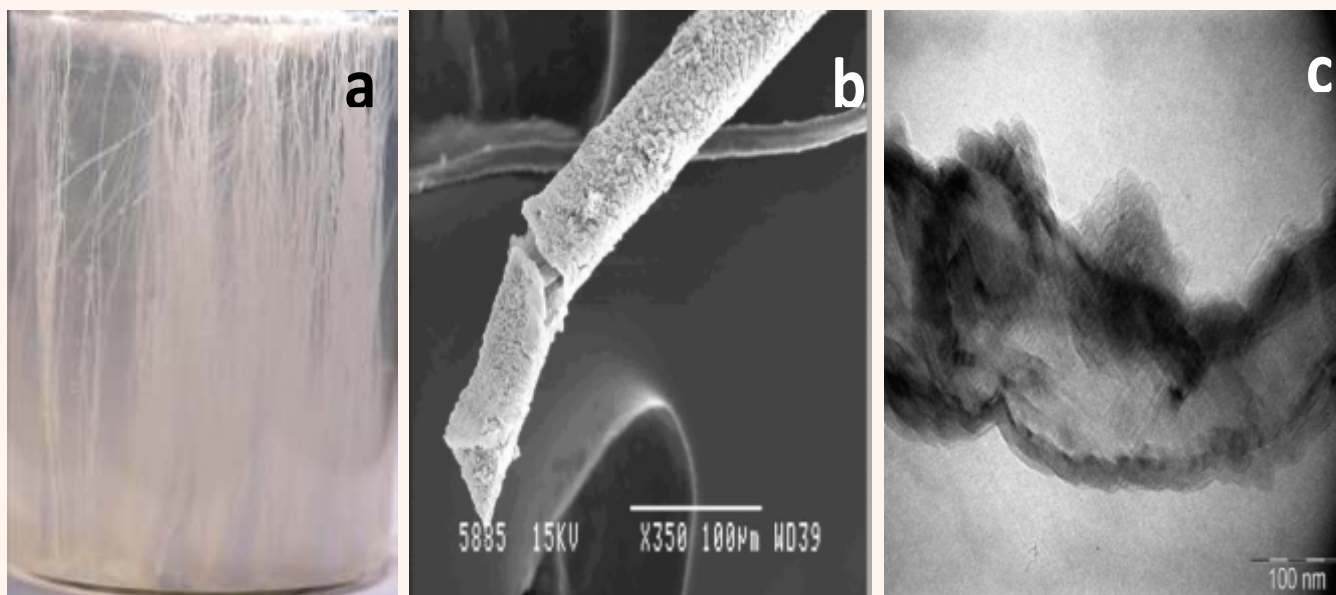
Fig.1. (a) CaSPT grown in the laboratory, (b) SEM image of 'as grown' CaSPT, (c) TEM image of crushed particle of CaSPT at higher magnification.
