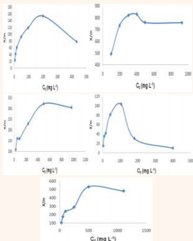
Figure 7. Plot of Loading capacity of Zn(II), Pb(II), Cd(II) Cu(II) and Cr(III)
