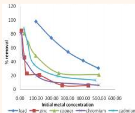
Figure 4. Effect of metal ion concentration on cation adsorption
