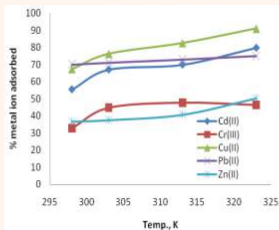
Figure 6. Effect of temperature on cation adsorption.
