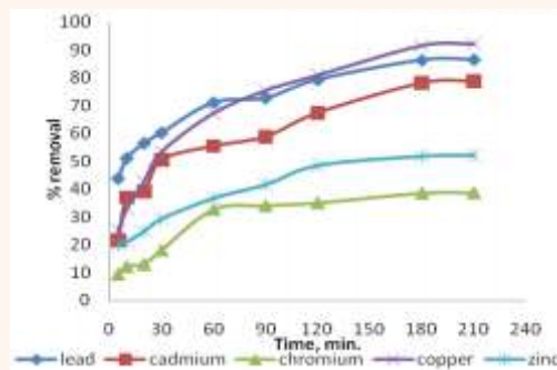
Figure 2: Effect of contact time on cation adsorption.
