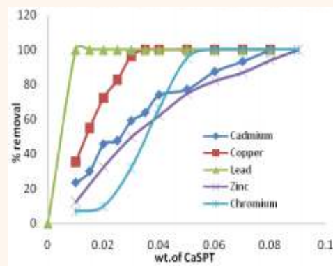
Figure 3. Effect of adsorbent dose on cation adsorption.
